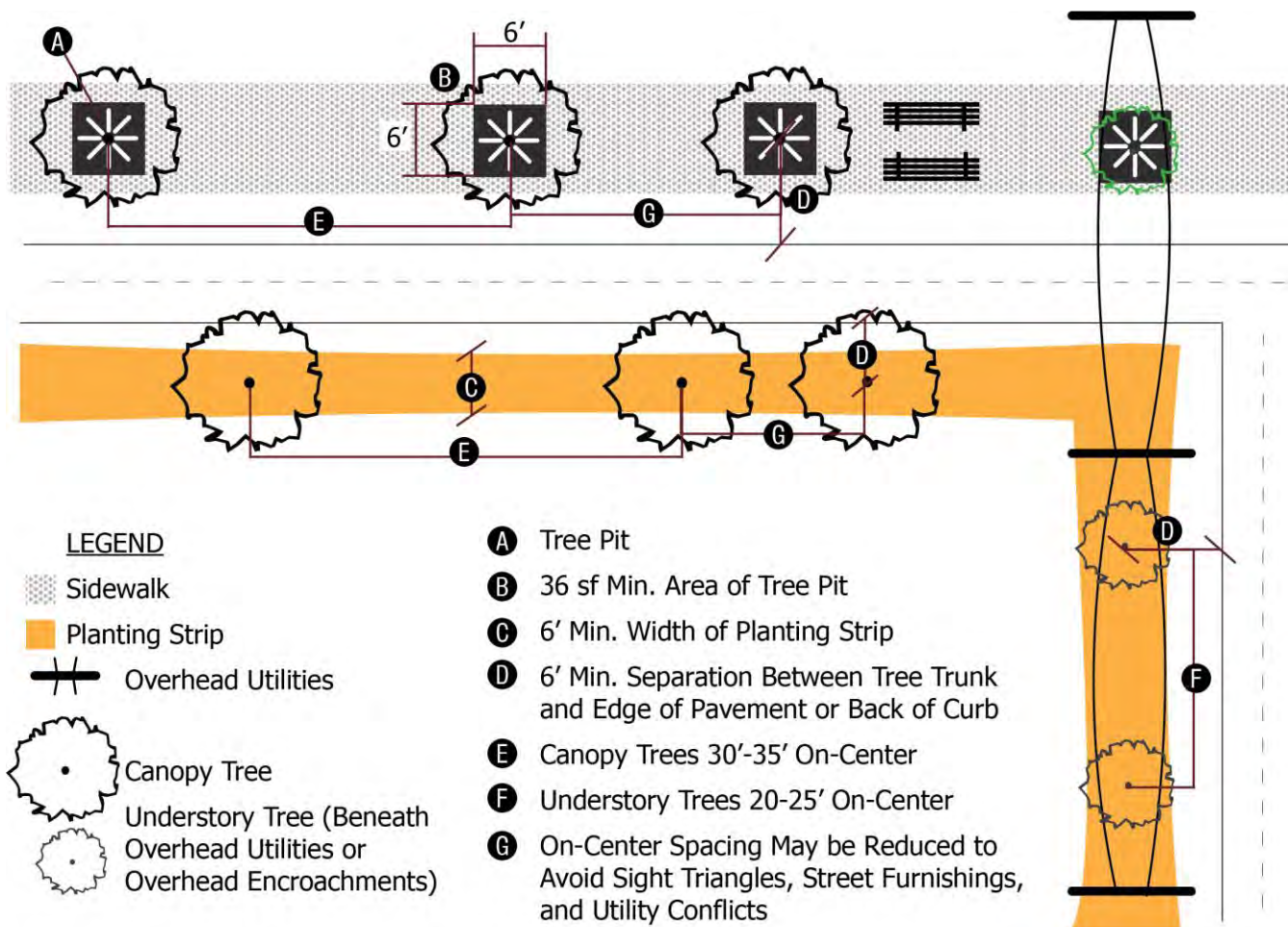
FIGURE 6.6.15: STREET TREE CONFIGURATION
