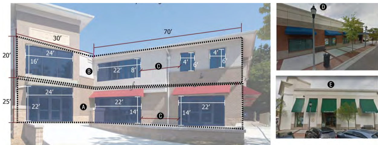
FIGURE 6.2.5.F.8: NON-RESIDENTIAL BUILDING FENESTRATION
