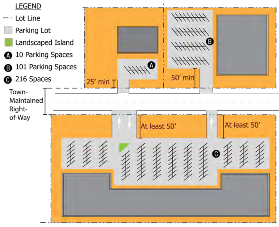
FIGURE 6.1.4.E: PARKING LOT ACCESSWAY DEPTH
