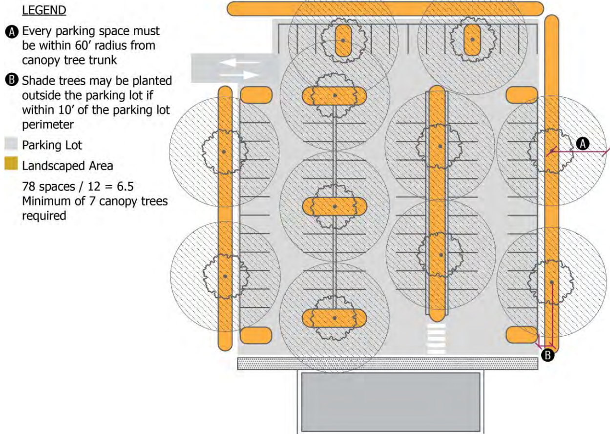
FIGURE 6.6.11.C: PARKING LOT SHADING
