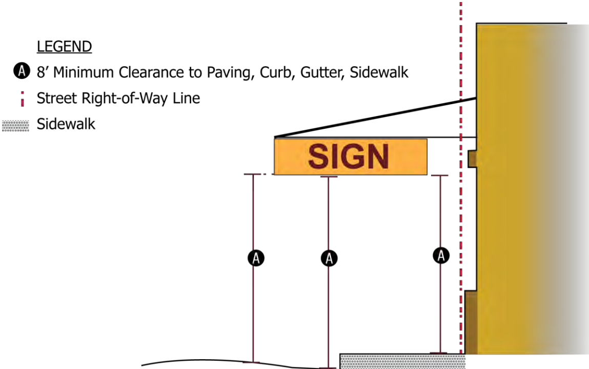
FIGURE 6.13.7: MINIMUM VERTICAL CLEARANCE
