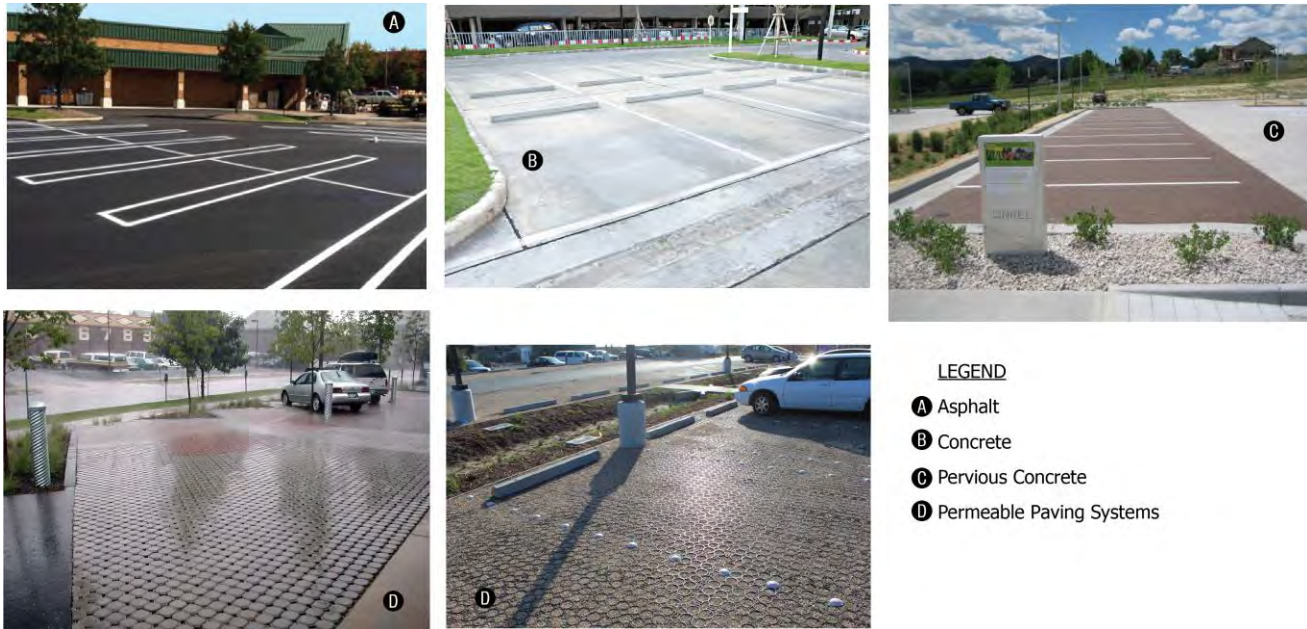
FIGURE 6.9.7.M: PARKING LOT SURFACE MATERIALS
